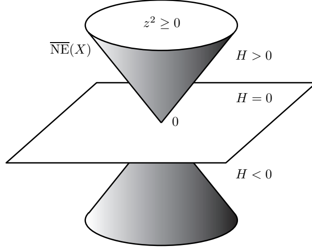
The effective cone of an abelian surface X
