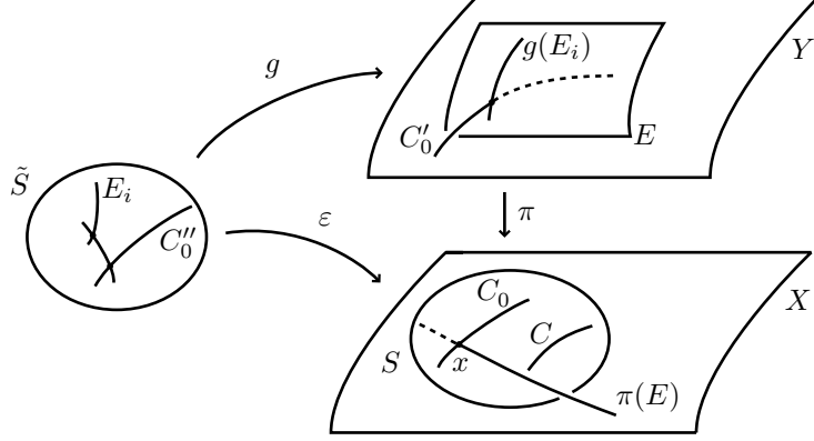
Construction of a rational curve g(E_i) in the exceptional locus E of \pi
